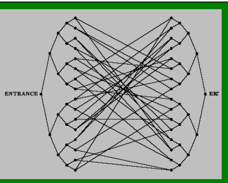
Graphs for quantum walks
