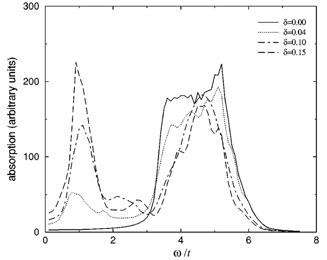
FIG. 24. Optical absorption (arbitrary units) as a function of the frequency (in units of t ) for various dopings. The Hubbard parameter is U/t=5 and the corresponding self-consistent lowest-energy configurations of frozen liquids of merons and antimerons were used. The damping coefficient is \Gamma=0.1t . As the doping increases, a broadband due to electronic excitations from the lower Mott-Hubbard gap to the discrete, empty, meron-induced levels develops deep in the gap.
