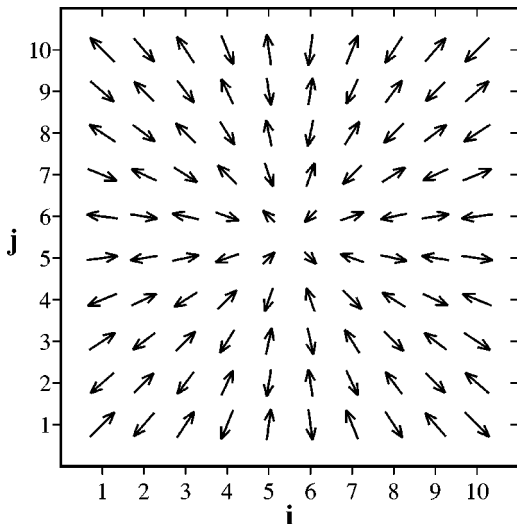
FIG. 9. Self-consistent spin distribution of a 10 \times 10 lattice with a meron vortex in the spin-flux phase. The core of the meron is localized in the center of a plaquette, in the spin-flux phase (in the conventional phase, the core of the meron vortex is localized at a site). This excitation has a topological winding number 1 since the spins on either sublattice rotate by 2\pi on any curve surrounding the core. The magnitude of the staggered magnetic moments is slightly diminished near the vortex core, but is equal to that of the undoped AFM background far from the core.
