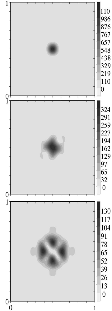
FIG. 25. Static magnetic structure factor as a function of (k_x, k_y) , measured in units of 2\pi/a . The first picture corresponds to \delta=0.00 and has the large magnetic peak at (\pi/a, \pi/a) . As the doping increases to \delta=0.05 (second picture) and \delta=0.08 (third picture) this magnetic peak splits into four incommensurate satellites. The Hubbard parameter is U/t=5 and the corresponding self-consistent lowest-energy configurations of frozen liquids of merons and antimerons were used.
