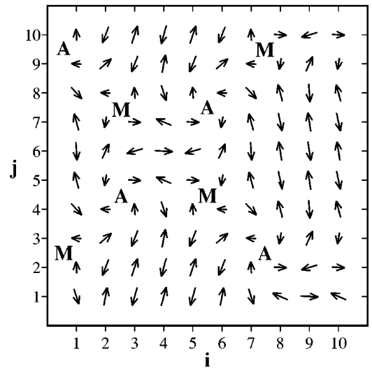
FIG. 19. Self-consistent spin distribution for the configuration of lowest energy found at \delta = 0.08 (eight holes), starting from an initial random distribution, for U/t = 5 in the spin-flux phase. Four meron-antimeron pairs appear. We have marked with M the plaquettes on which merons are centered and with A the plaquettes on which antimerons are centered. A meron and an antimeron are “split” between the two opposing boundaries (we have imposed cyclic boundary conditions).
