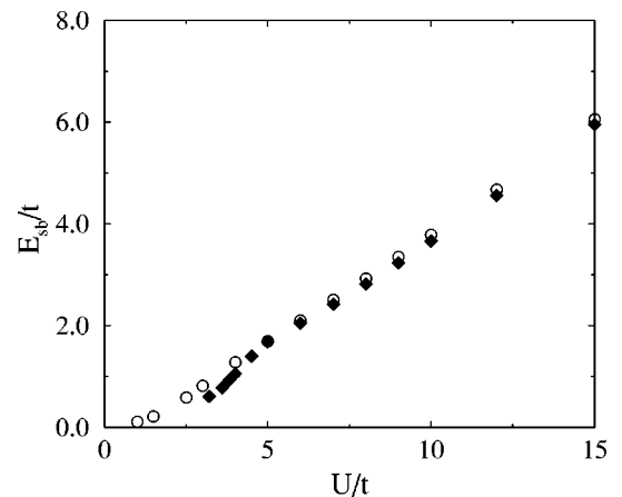
FIG. 8. Excitation energy of a spin bag E_{spin\ bag} as a function of U/t , in the presence of spin flux (filled diamonds) and in the conventional state (circles). In the very large U/t limit, the excitation energy approaches asymptotically the value U/2-2t . The excitation energy of a spin bag is lower in the spin-flux phase than in the conventional phase.
