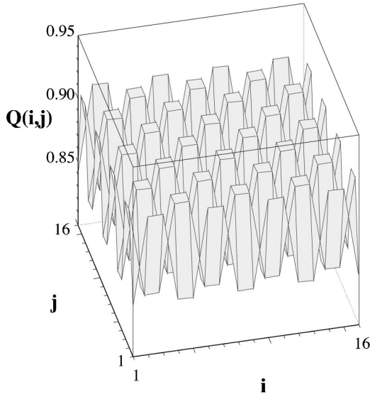
FIG. 22. Self-consistent charge distribution for the configuration of lowest energy found at \delta=1/8 for U/t=5 in the spin-flux phase. An ordered crystal of charged merons and antimerons is created.
