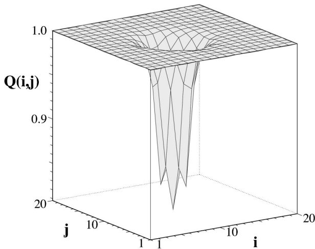
FIG. 17. Self-consistent charge distribution for a tightly bound meron-antimeron pair. The doping charge is mostly localized on the two plaquettes containing the meron and antimeron cores. Due to interactions, the cores of the vortices are somewhat distorted, with most of the charge missing from the (10,10) site common to both cores. The two holes localized in the cores are responsible for the fact that the meron-antimeron pair does not collapse (due to Fermi statistics, it is impossible to have two holes at the same site).
