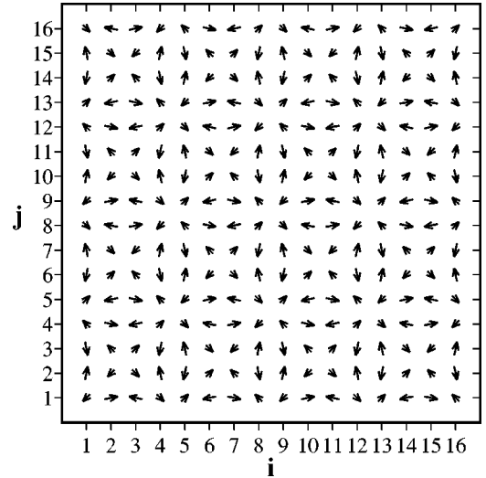
FIG. 21. Self-consistent spin distribution for the configuration of lowest energy found at \delta=1/8 for U/t=5 in the spin-flux phase. An ordered crystal of charged merons and antimerons is created.
