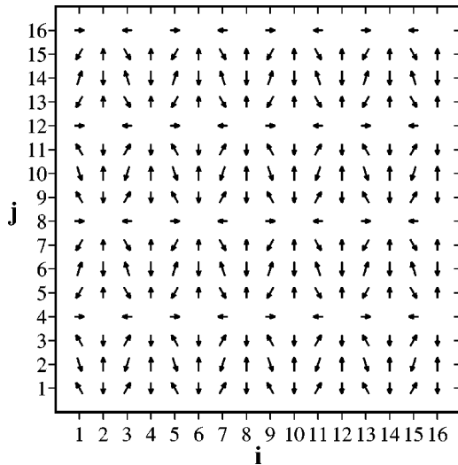
FIG. 23. Self-consistent spin distribution for the configuration of lowest energy found after adding a 3% anisotropy in the hopping integral, at \delta=1/8 , for U/t=5 in the spin-flux phase. The merons and antimerons rearrange on horizontal lines, leading to a structure similar to that suggested by Tranquada et al. in Ref. 32.
