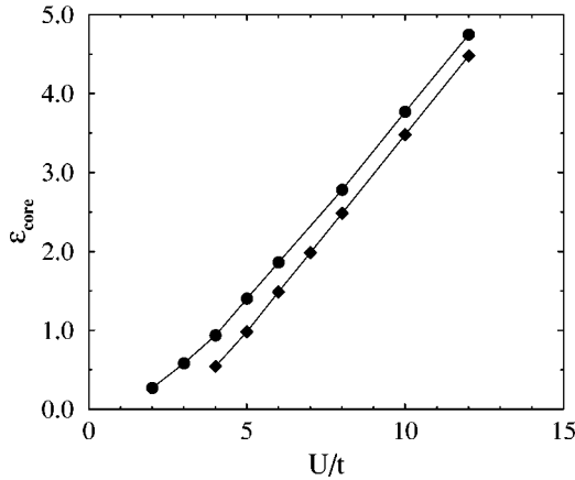
FIG. 14. Dependence of \epsilon_{core} (in units of t ) from the fit E_{meron}(N) = \alpha \ln N + \epsilon_{core} on U/t . Diamonds show results for a spin-flux phase, while circles correspond to a conventional state. The line serves to guide the eye. In the large U/t limit \epsilon_{core} \rightarrow E_{spin\ bag} since in this limit all spin configurations become degenerate and the excitation energy of the meron vortex should equal the excitation energy of the spin bag.
