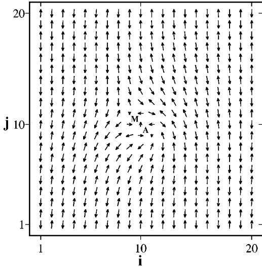
FIG. 16. Self-consistent spin distribution for a tightly bound meron-antimeron pair in the spin flux phase. The meron ( M ) and the antimeron ( A ) are localized on neighboring plaquettes. The total winding number of the pair is zero. The magnetic AFM order is disturbed only on the small region where the vortices are localized. The attraction between holes is of topological nature and on a long length scale is stronger than unscreened Coulomb repulsion between charges.
