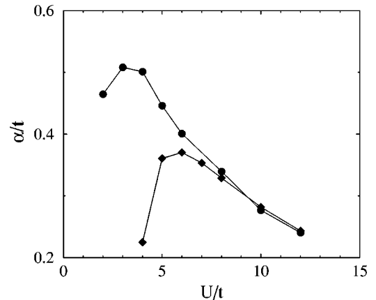
FIG. 13. Dependence of the coefficient \alpha (in units of t ) from the fit E_{\text{meron}}(N) = \alpha \ln N + \epsilon_{\text{core}} on U/t . Diamonds show results for a spin-flux phase, while circles correspond to a conventional state. The line serves to guide the eye. In the large U/t limit \alpha \rightarrow 0 since in this limit all spin configurations become degenerate and the excitation energy of the meron vortex should equal the excitation energy of the spin bag.
