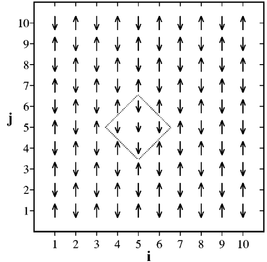
FIG. 4. Self-consistent spin distribution of a 10\times 10 lattice with a spin bag centered at (5,5). The spin bag has a small ferromagnetic core and the magnetic order is only locally affected.
