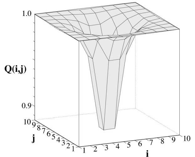
FIG. 10. Self-consistent charge distribution of a 10 \times 10 lattice with a meron vortex in the spin-flux phase. Most of the doping charge is localized in the center of the meron. Far from the core, there is an average of one electron per site.
