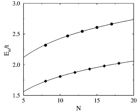
FIG. 12. Excitation energy (in units of t ) of a single meron vortex, as a function of the meron size N , in the presence of the spin flux (diamonds) and without spin flux (circles). The lines show fits with a logarithmic dependence on N , E_{\text{meron}}(N) = \alpha \ln N + \epsilon_{\text{core}} . The excitation energy of a meron vortex is always lower in the spin-flux phase than in the conventional phase. If the size of the meron core is small enough, the excitation energy of the meron vortex may become smaller than the excitation energy of a spin bag.
