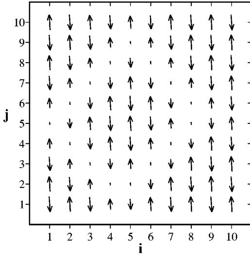
FIG. 20. Self-consistent spin distribution for the configuration of lowest energy found at \delta=0.15 , starting from initial random distributions, for U/t=5 in the conventional phase. A closed charged stripe appears (cyclic boundary conditions were imposed). The AFM order is switched from one phase to the other one (up to down and vice versa) as the stripe is crossed.
