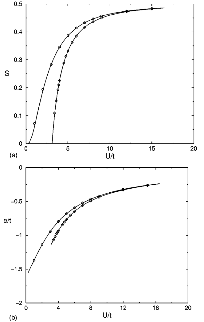
FIG. 3. (a) Dependence of the staggered spin S of the AFM undoped compound with U/t . The diamonds show the numerical results obtained in the presence of the spin flux, while circles show numerical results for the conventional phase. The lines show the values predicted by Eqs. (6) and (9) for the two phases. The spin-flux phase has a mean-field AFM solution ( S \neq 0 ) only for U/t > 3 . As expected, S \rightarrow 1/2 in the large U/t limit, where every electron becomes localized on individual sites. (b) Dependence of the ground-state energy per site of the AFM parent compound with U/t . The diamonds show the numerical results obtained in the presence of the spin flux, while circles show numerical results for the conventional phase. The lines show the values predicted by Eqs. (5) and (8) for the two phases. The mean-field AFM spin-flux phase has a lower energy than the mean-field AFM conventional phase for all values of U/t .
