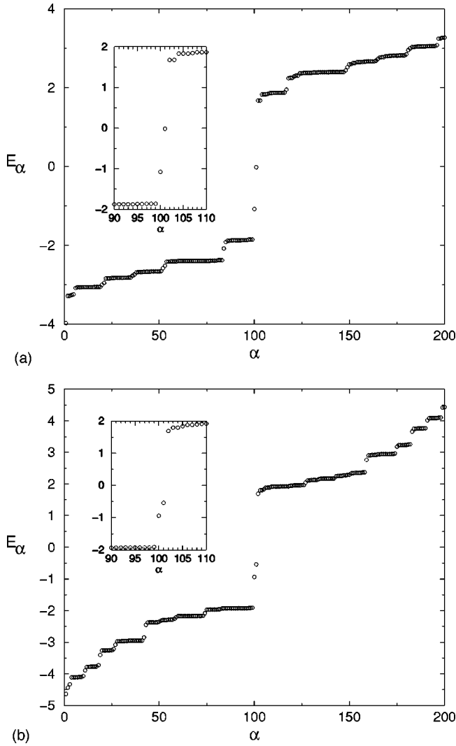
FIG. 6. (a) Electronic spectrum of a spin bag on a 10 \times 10 lattice for U/t=5 and spin flux. Eigenenergies E_\alpha are plotted as a function of \alpha=1, 2, \dots, 2N^2 ( N=10 ). Only the first N^2-1=99 states are occupied. There are two empty bound discrete levels deep into the Mott-Hubbard gap ( \alpha=100, 101 ), one of which comes from the valence band of the undoped AFM compound (see inset). There is also an occupied discrete level below the valence band ( \alpha=1 ). The valence band is spin paired since it has an even number of levels. Thus the total spin of the spin bag comes from the discrete occupied level. The spin bag is a charged, spin- \frac{1}{2} fermion. (b) Electronic spectrum of a spin bag on a 10 \times 10 lattice for U/t=5 in the conventional state. Eigenenergies E_\alpha are plotted as a function of \alpha=1, 2, \dots, 2N^2 ( N=10 ). Only the first N^2-1=99 states are occupied. There are two empty bound discrete levels deep into the Mott-Hubbard gap ( \alpha=99, 100 ), one of which comes from the valence band of the undoped AFM compound (see inset). There are also three occupied discrete levels below the valence band ( \alpha=1, 2, 3 ). The valence band is spin paired since it has an even number of levels. Thus the total spin of the spin bag comes from the discrete occupied levels. The spin bag is a charged, spin- \frac{1}{2} fermion.
