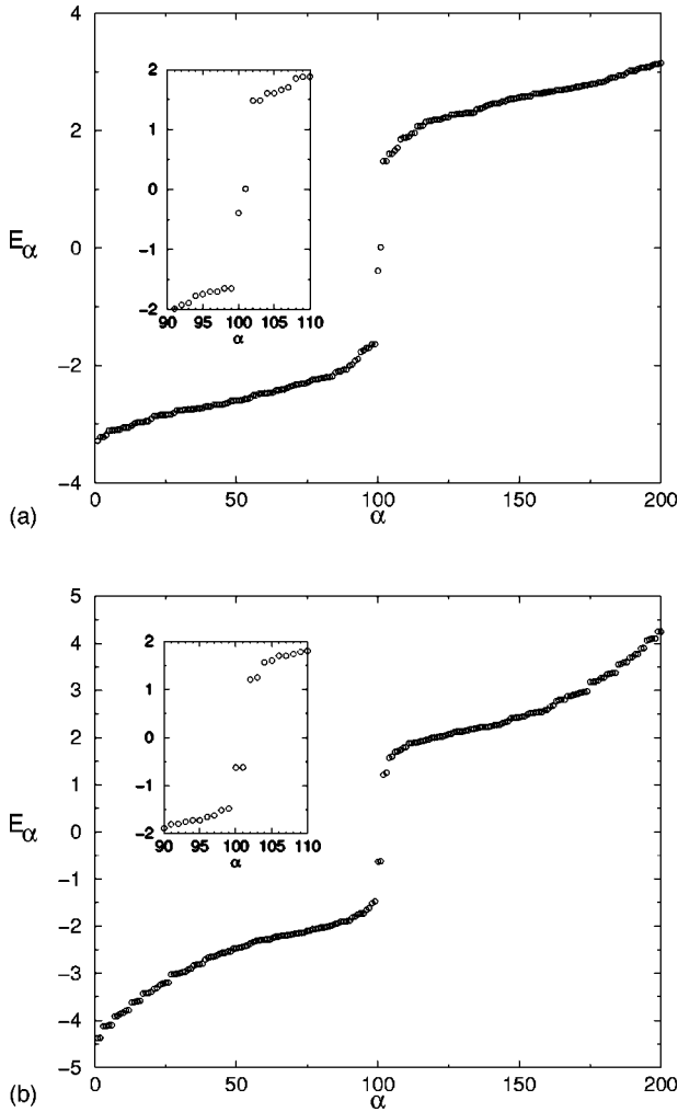
FIG. 11. (a) Electronic spectrum of a meron vortex on a 10 \times 10 lattice, for U/t=5 , in the presence of the spin flux. Eigenenergies E_\alpha are plotted as a function of \alpha = 1, 2, \dots, 2N^2 ( N=10 ). Only the first N^2-1=99 states are occupied (the valence band). There are two discrete empty levels deep into the Mott-Hubbard gap, one of which ( \alpha=100 ) comes from the valence band of the undoped AFM parent. Merons must be created in vortex-antivortex pairs (for topological reasons). Each pair removes two levels from the undoped AFM valence band. Thus the valence band remains spin paired and the total spin of this excitation is zero. This meron is a spinless, charged, bosonic collective excitation of the doped antiferromagnet. (b) Electronic spectrum of a meron vortex on a 10 \times 10 lattice, for U/t=5 , in the conventional phase. Eigenenergies E_\alpha are plotted as a function of \alpha = 1, 2, \dots, 2N^2 ( N=10 ). Only the first N^2-1=99 states are occupied (the valence band). There is a double degenerate unoccupied bound discrete level deep into the Mott-Hubbard gap. One of these bound levels ( \alpha=100 ) comes from the valence band of the undoped AFM parent. Merons must be created in vortex-antivortex pairs (for topological reasons). Each pair removes two levels from the undoped AFM valence band. Thus the valence band remains spin paired and the total spin of this excitation is zero.
