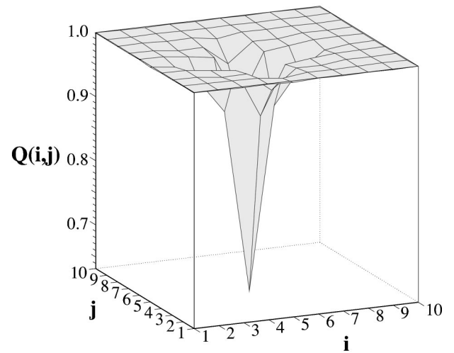
FIG. 5. Self-consistent charge distribution of a 10\times 10 lattice with a spin bag centered at (5,5). There is an average of one electron per site everywhere, except in the core of the spin bag, where the doping hole is localized.
