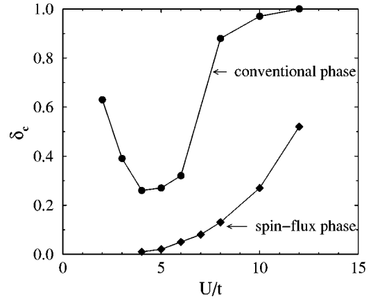
FIG. 15. Critical doping concentration \delta_c , above which a charged meron-antimeron liquid is energetically favorable compared to a gas of spin bags. Diamonds show results for a spin-flux phase, while circles correspond to a conventional state. The line serves to guide the eye. In the conventional phase the critical concentrations are very large, \delta_c > 0.3 . In the spin-flux phase the transition to the liquid of meron vortices takes place at dopings smaller than 0.10 for U/t < 8 . In the conventional phase the critical doping is so large ( \delta_c > 0.30 ) that merons are unlikely to appear before the Mott-Hubbard gap itself closes.
