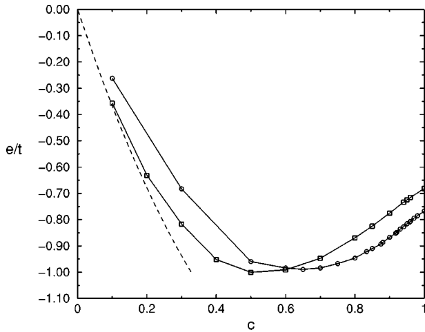
FIG. 18. Energy per site (in units of t ) as a function of the electron concentration c = 1 - \delta for U/t = 5 . Circles correspond to the lowest energies found in the random trial in the spin-flux phase (liquid of meron vortices), while squares correspond to the best result of the random trial in the conventional phase (stripes). The dashed line shows the exact value for U = 0 (noninteracting case). At low doping (high electron concentration) the liquid of meron vortices of the spin-flux phase has a lower energy than the stripes of the conventional phases. However, at higher dopings ( \delta > 0.4 ) the conventional phase becomes stable.
