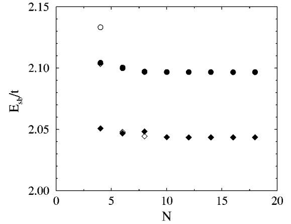
FIG. 7. Excitation energy of a spin bag E_{spin\ bag} as a function of the lattice size N . Diamonds show results for a spin-flux AFM phase, with CBC's (full diamonds) and FBC's (empty diamonds). Circles show results for the conventional AFM state, with CBC's (full circles) and FBC's (empty circles). The Hubbard parameter is U/t=6 . The bulk limit is reached for N>10 . In this limit, the excitation energy of the localized spin bag becomes independent of the size of the lattice.
