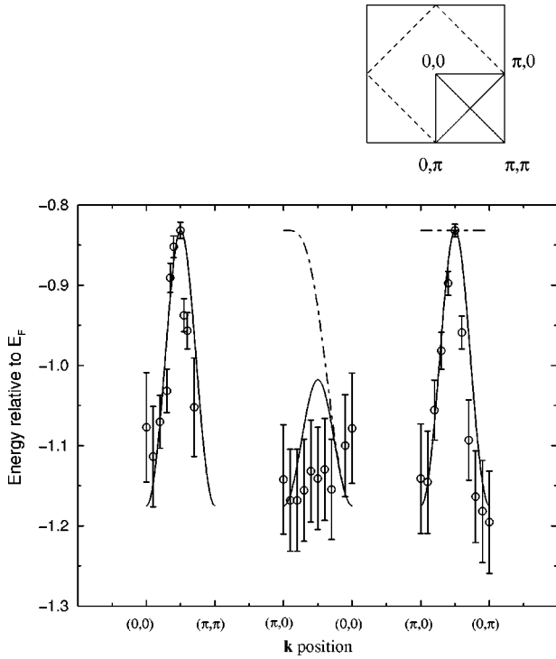
FIG. 2. Comparison between the experimentally determined E(\vec{k}) quasiparticle dispersion relation, from angle resolved photoemission studies (ARPES), for the insulating \text{Sr}_2\text{CuO}_2\text{Cl}_2 (open circles with error bars) and the mean-field AFM spin-flux phase dispersion relation (full line) and the mean-field AFM conventional phase dispersion relation (dash-dotted line). While the peak on the (0,0) to (\pi, \pi) is equally well described in both models, the mean-field spin-flux model gives a much better agreement for the (\pi, 0) to (0,0) and (\pi, 0) to (0, \pi) directions. The fitting corresponds to U = 2.01 eV and t = 0.29 eV for the spin-flux phase and U = 1.98 eV and t = 0.21 eV for the conventional phase. The experimental results are the ARPES results of Ref. 21.
